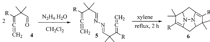
Scheme 4. Intramolecular criss-cross cycloaddition of azines.
