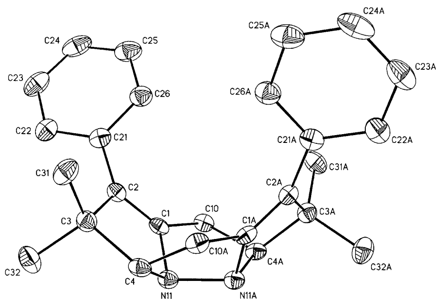
Figure 3. A perspective view of 3,3,8,8-tetramethyl-2,7-diphenyl-11,12-diazatetracyclo[4.4.2.0 4,11 .0 9,12 ]dodeca-1,6-diene ( 6g ) showing the dish-like shape of the central heterocyclic moiety. The atoms marked with the A suffix are generated by rotation through the two-fold symmetry axis that bisects the N11–N11A linkage and lies in the plane of paper.
