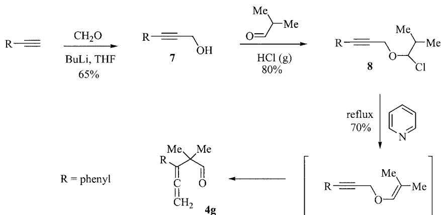
Scheme 3. Preparation of allenyl aldehyde 4g .
