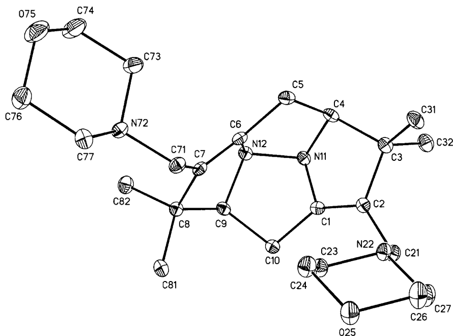
Figure 1. A perspective view of 3,3,8,8-tetramethyl-2,7-bis(morpholin-4-ylmethyl)-11,12-diazatetracyclo[4.4.2.0 4,11 .0 9,12 ]dodeca-1,6-diene ( 6e ).
